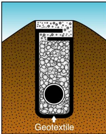
Drainage
